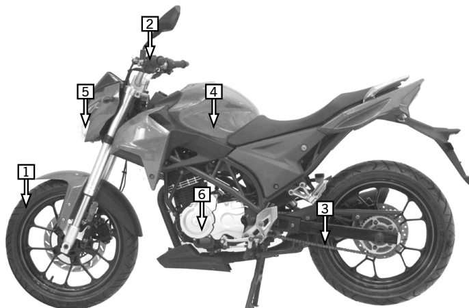
Figure 1-3 General Construction Chart of a Complete Motorcycle
