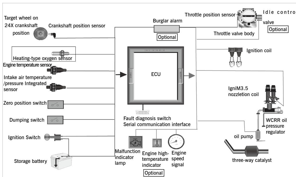
Structural Schematic Diagram for EFI System
