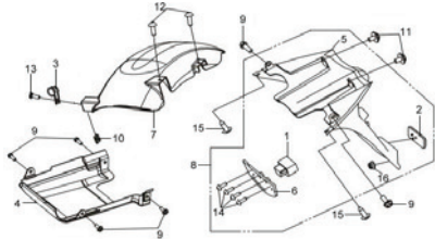
F12 RR. FENDER ASSY
