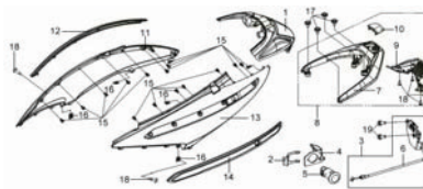
F08 BODY COVER & TAIL LIGHT
