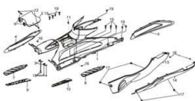
F10 FLOOR PANEL & SIDE COVER
