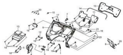
F09 SEAT & LUGGAGE BOX
