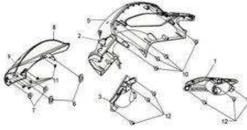
F05 FR. COVER & FR. COVER
