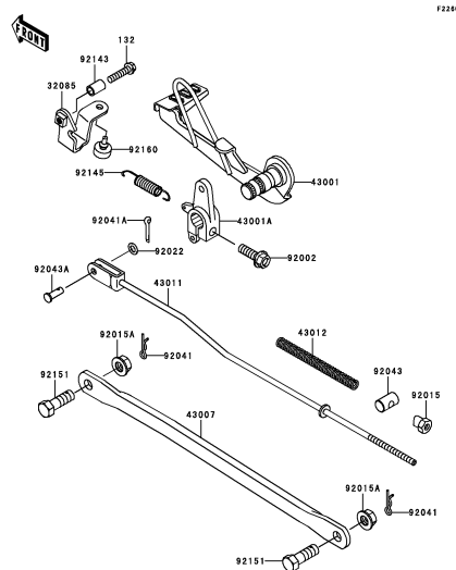
E-7 Brake Pedal(M6F)
