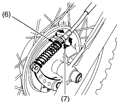
(6) lower lock nut
