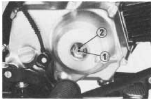
(1) Clutch adjuster
