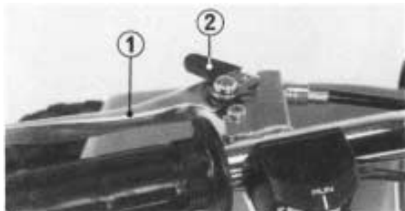
(1) Rear brake/Parking brake lever (2) Lock
