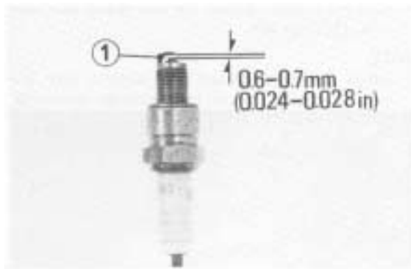
(1) Side electrode
