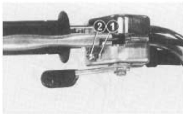
(1) Lock nut (2) Speed limiter screw
