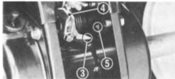
(3) Arrow (5) Reference mark (4) Brake arm
