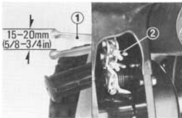
(1) Rear brake lever (2) Brake lever adjusting nut
