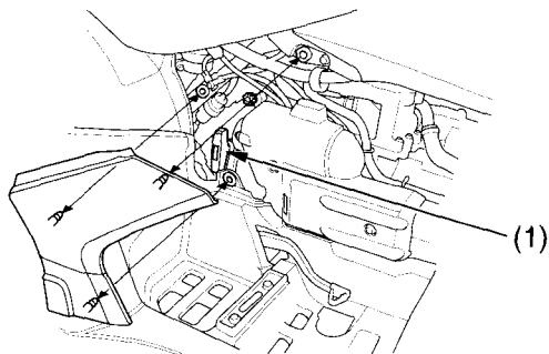
(1) recoil starter
