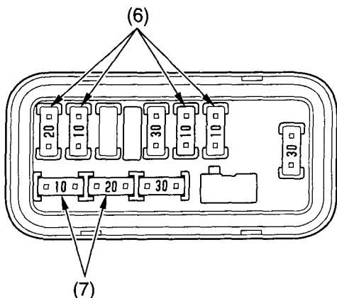
(6) circuit fuse
