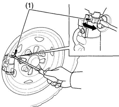
(1) brake shoe adjuster
