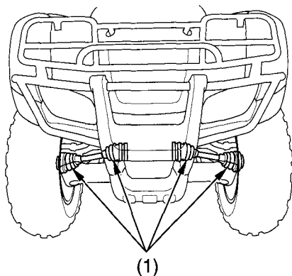
(1) driveshaft boots
