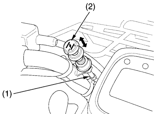
(1) choke cable
