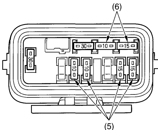
(6) spare fuses
