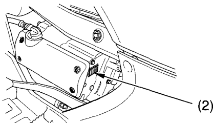
(2) engine number
