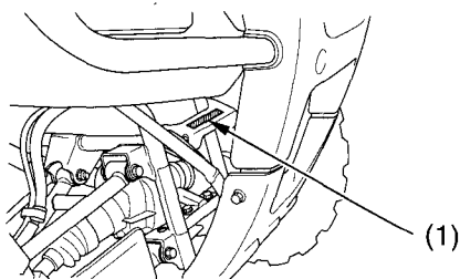
(1) frame number
