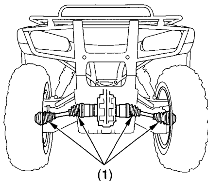
(1) driveshaft boots
