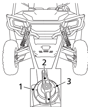
damping adjuster
