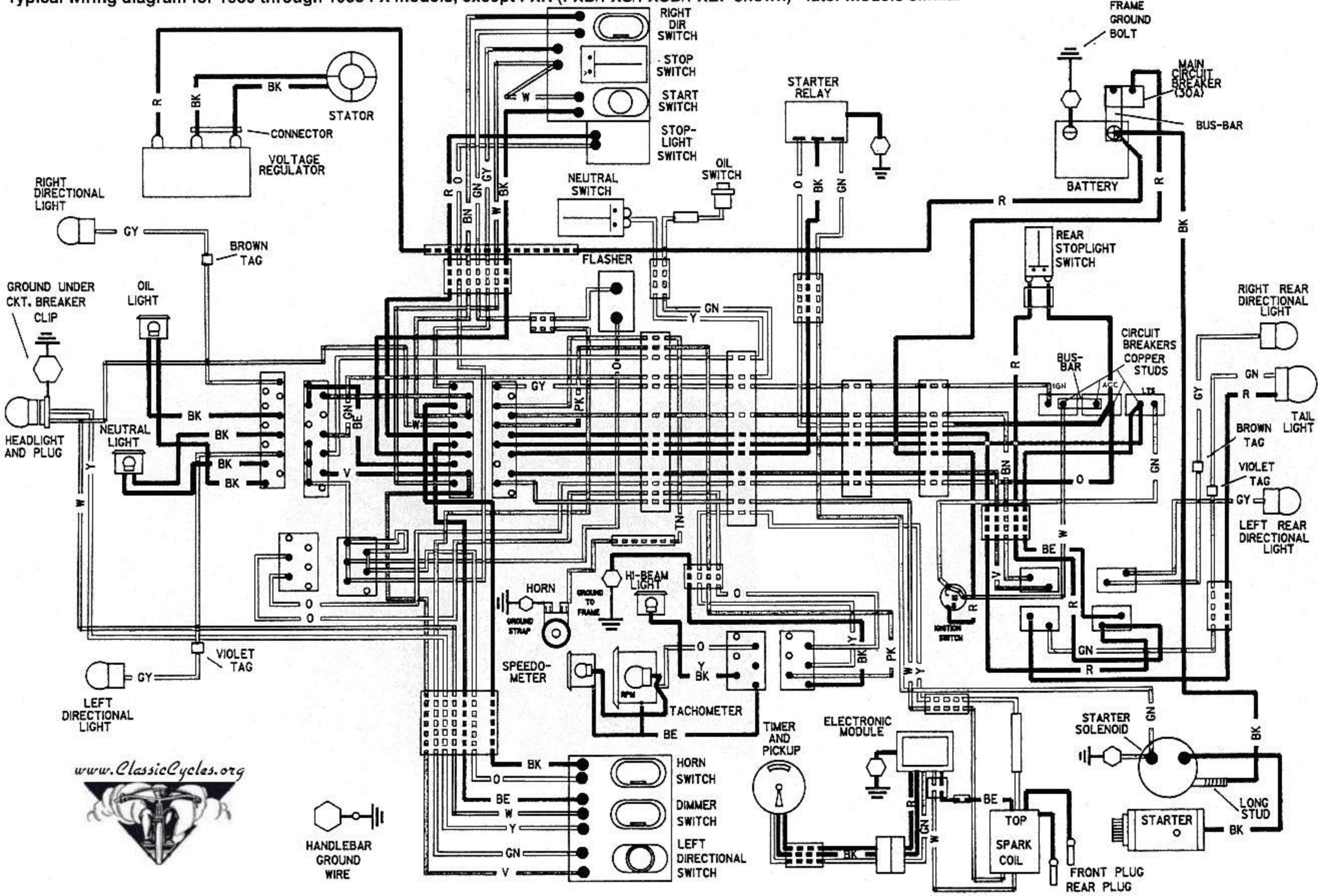
Typical wiring diagram for 1980 through 1983 FX models, except FXR (FXB/FXS/FXSB/FXEF shown) – later models similar
