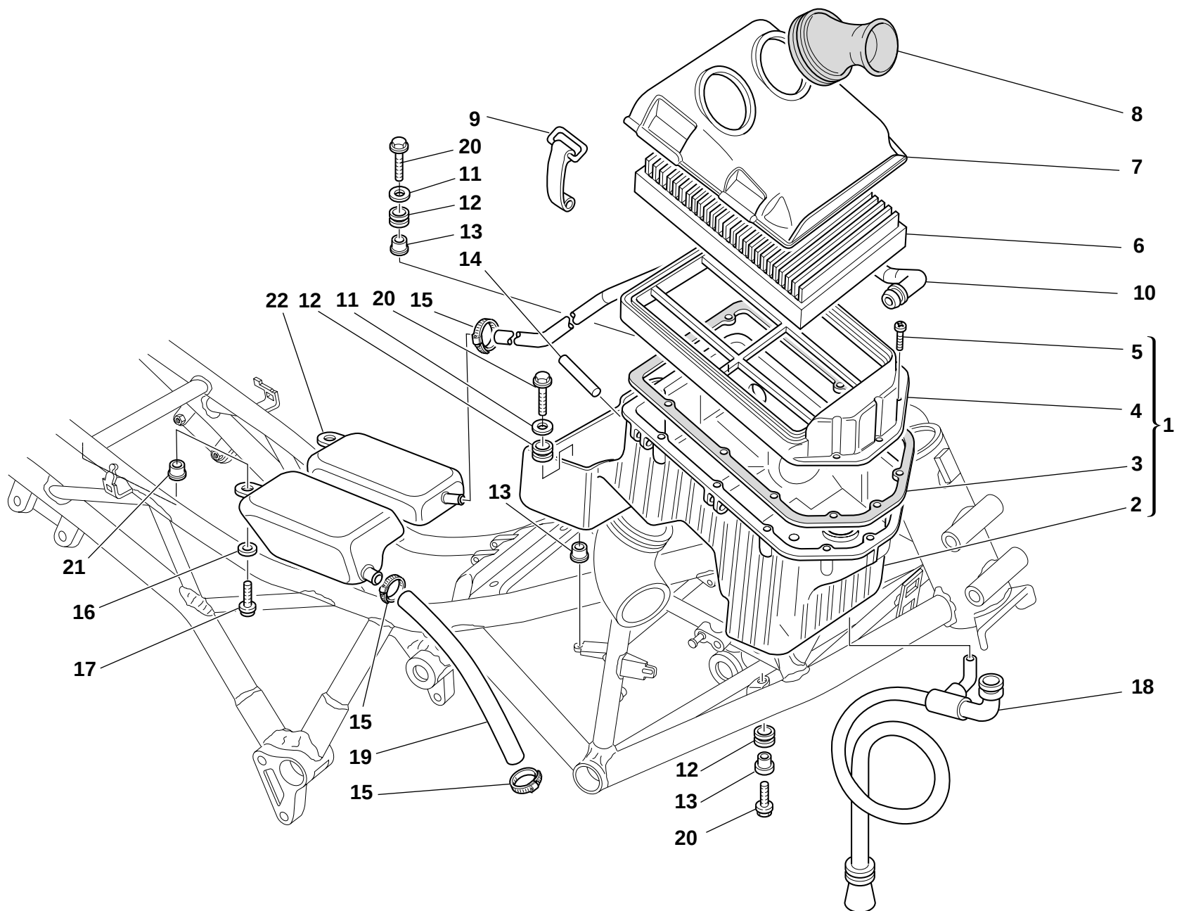
DRAWING 030 AIR INDUCTIO AND OIL VENT
