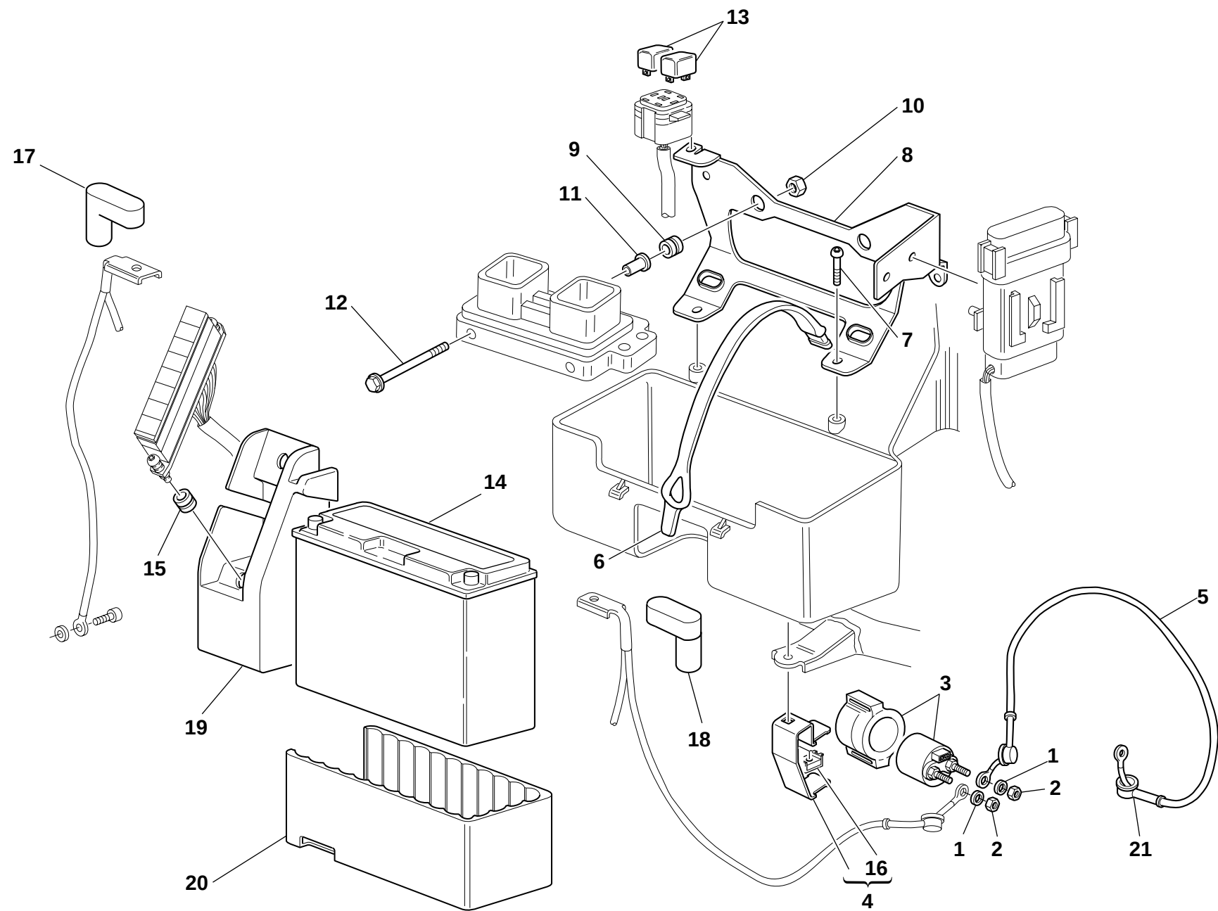
DRAWING 029 BATTERY BOX MOUNT
