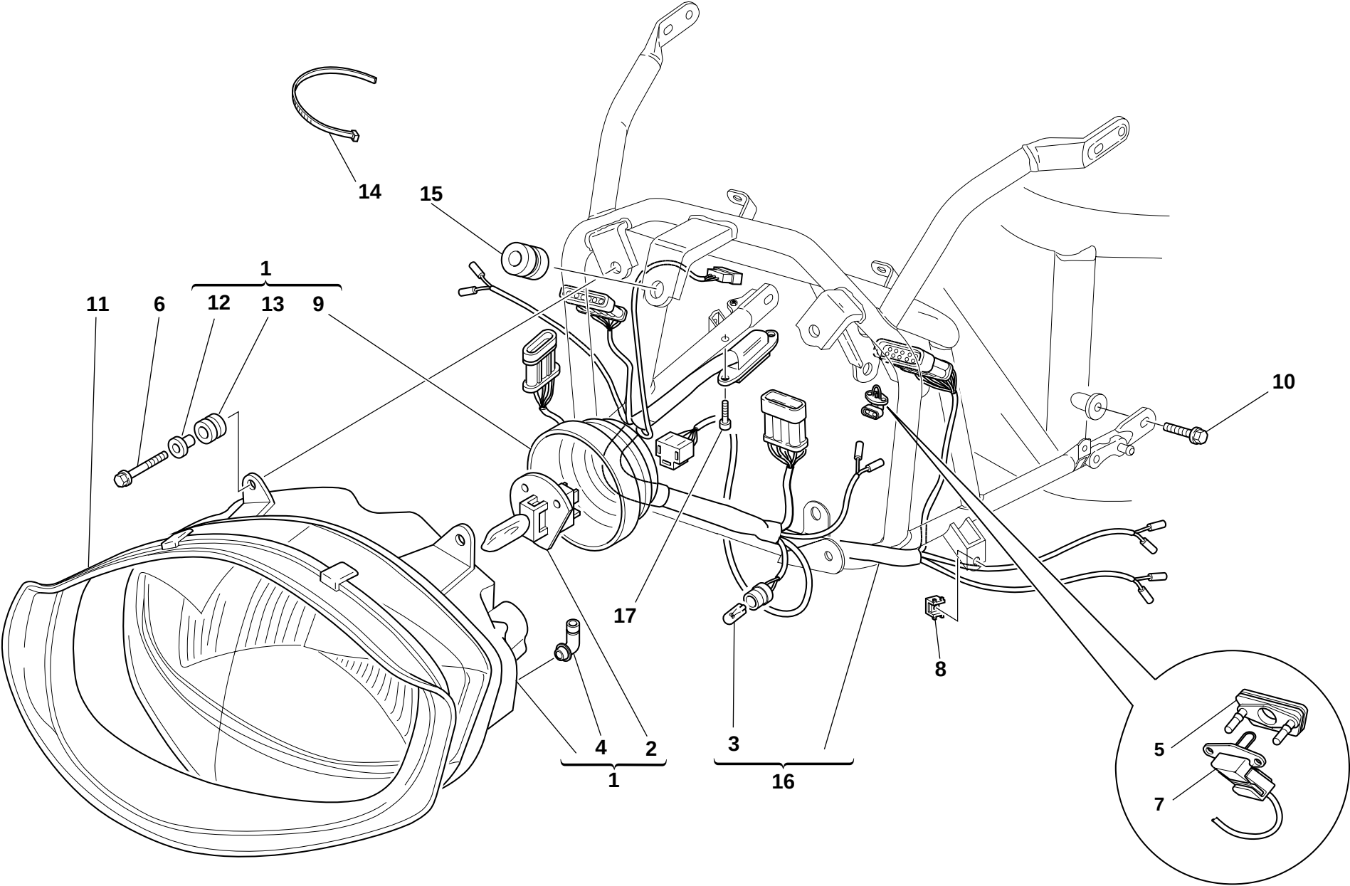
DRAWING 022 HEAD-LIGHT AND ELECTRIC WIRING
