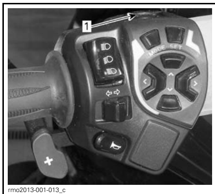
1. Reverse button
