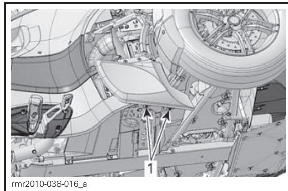
1. Plastic rivets
