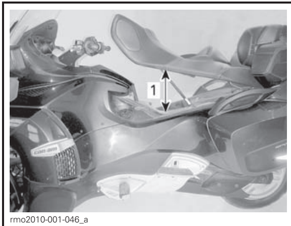
1. Maximum opening of seat
