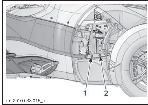
1. Upper retaining screw 2. Upper plastic rivet
