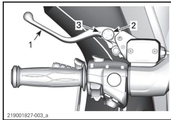
CLUTCH LEVER ADJUSTMENT
