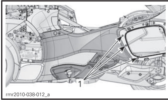
1. Rear retaining screws
