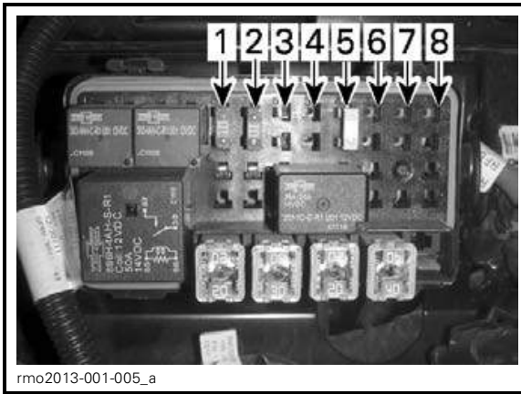
FUSES - RIGHT FUSE BOX
