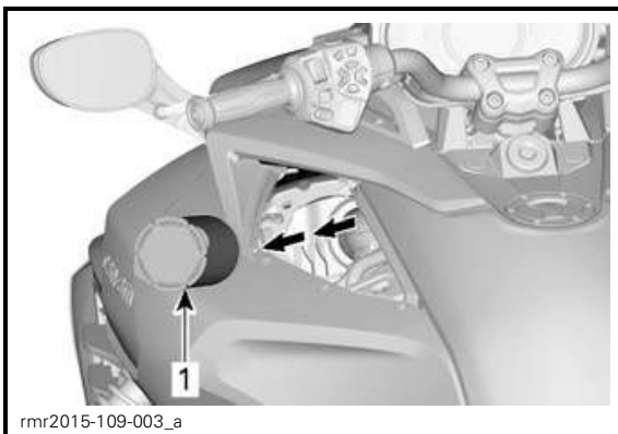
REMOVE AIR FILTER FROM AIR INTAKE SILENCER.
