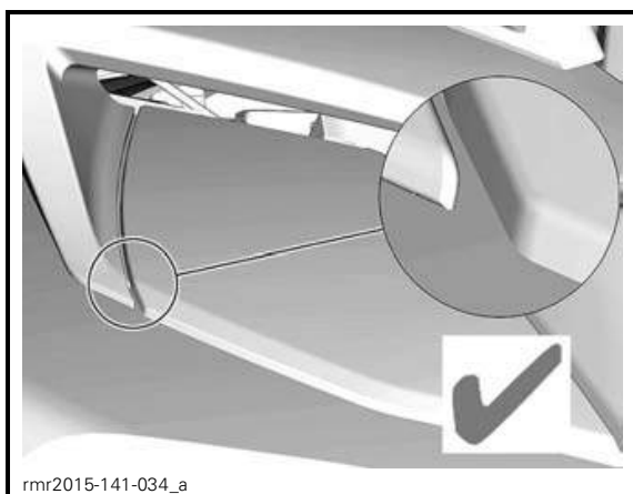
CORRECT INSTALLATION
