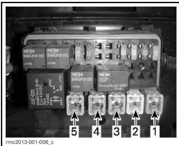
JCASE FUSES - LEFT FUSE BOX
