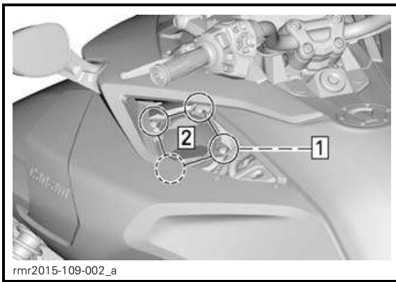
Step 1: Remove all four screws Step 2: Remove air filter cover
