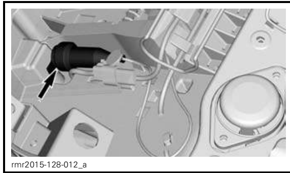
DC56 - REAR CUSTOMER ACCESSORY CIRCUIT - UNDER PASSENGER SEAT
