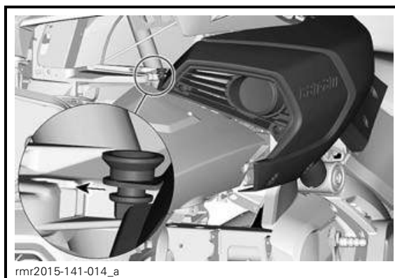
ALIGNING PANELS PROPERLY
