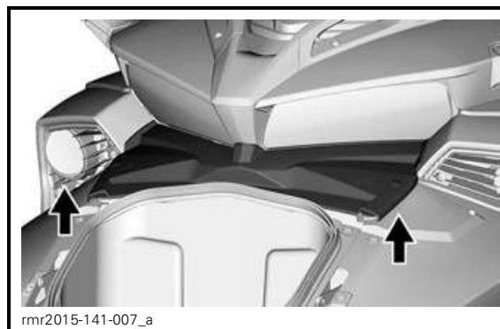
LIFTING SERVICE COVER
