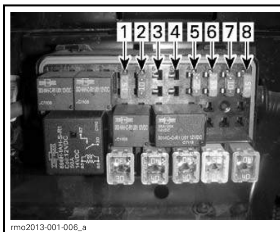
FUSES - LEFT FUSE BOX
