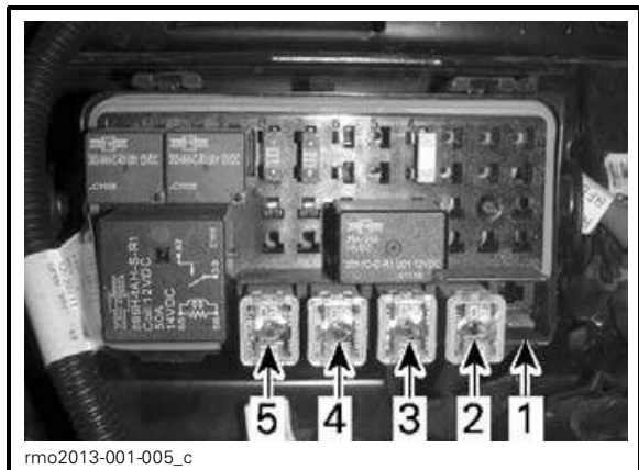
JCASE FUSES - RIGHT FUSE BOX
