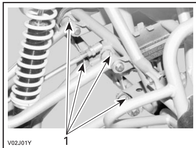
1. Grease fittings
