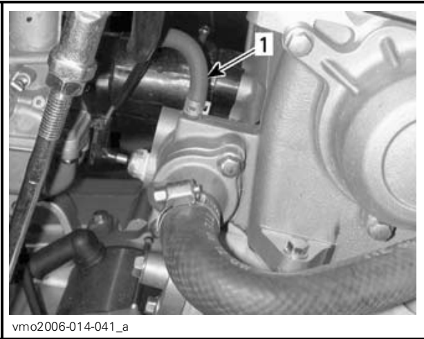
1. By-pass hose
