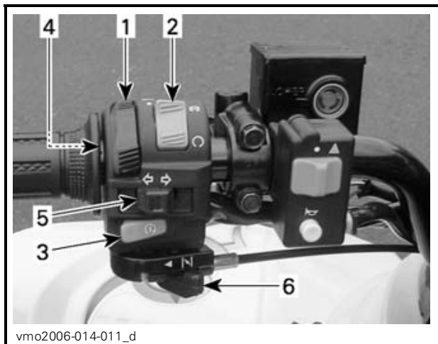
TYPICAL — MULTIFUNCTION SWITCH
