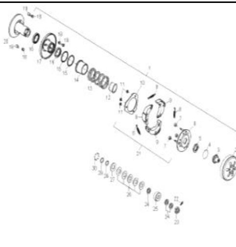
D-35: DRIVEN CLUTCH
