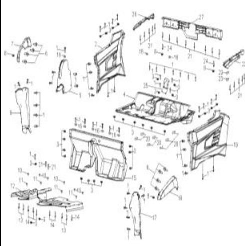
D-4: MOLDINGS
