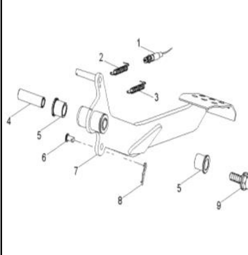
D-17: FOOT BRAKE
