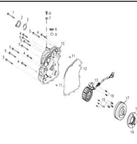
D-32: RIGHT CRANKCASE COVER
