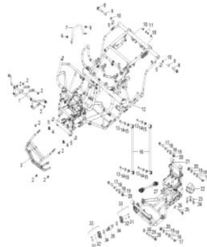
D-3: FRAME BODY
