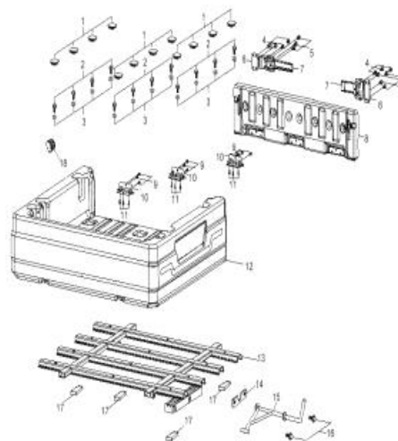
D-8: DUMP BOX
