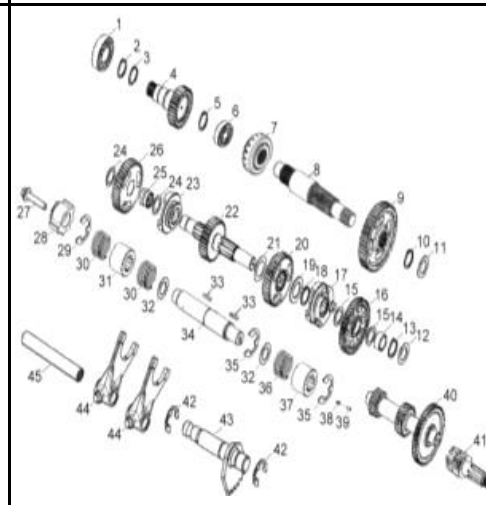
D-36: TRANSMISSION
