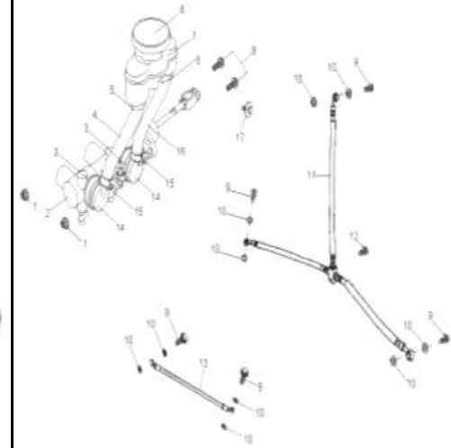
D-18: BRAKE LINES & MASTER CYLINDER
