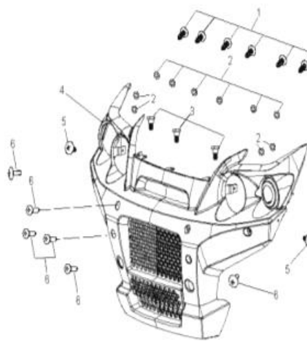
D-2: BUMPER
