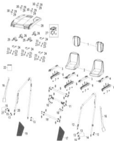
D-1: SEAT & CAGE
