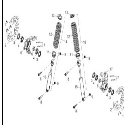
D-12: FRONT SHOCK
