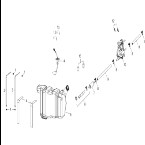
D-10: FUEL SYSTEM
