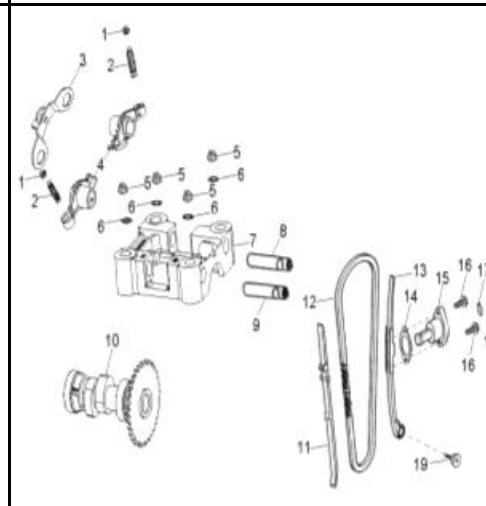
D-33: VALVE CAM
