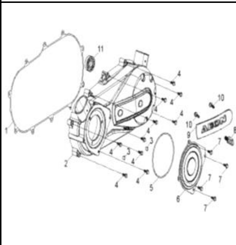
D-31: LEFT CRANKCASE COVER
