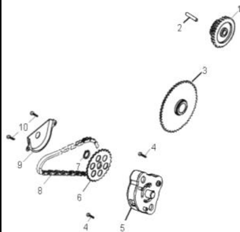
D-37: OIL PUMP
