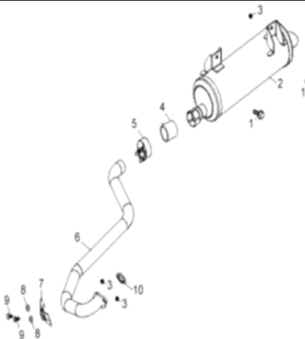
D-11: EXHAUST PIPE
