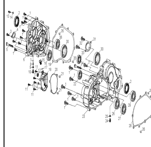
D-30: DRIVE ASSEMBLY REAR
