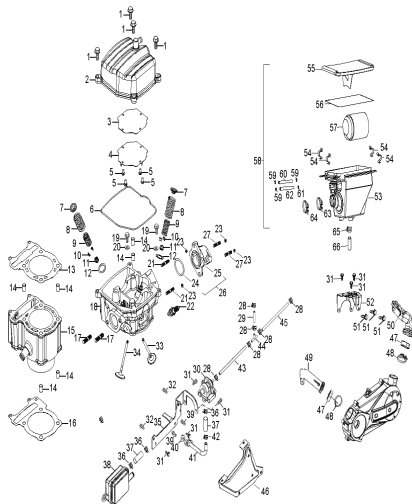
CYLINDER HEAD, DUAL INTAKE & AIR FI
