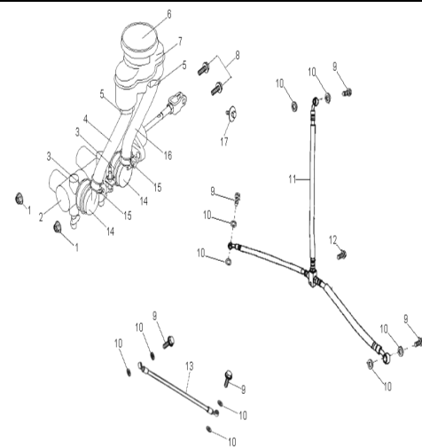
D-18: BRAKE LINES & MASTER CYLINDER
