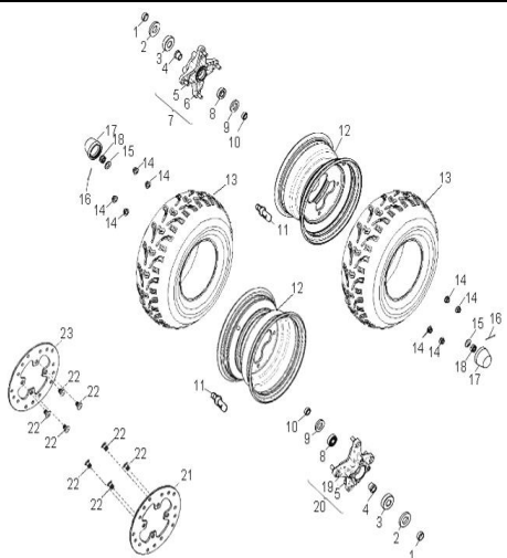
D-13: FRONT WHEEL
