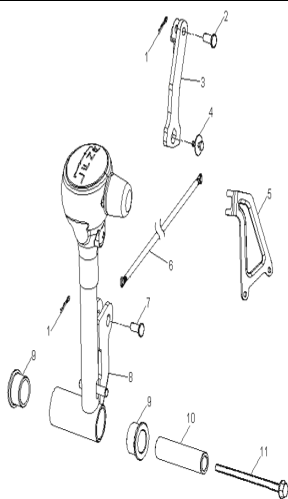
D-25: GEAR SELECTOR
