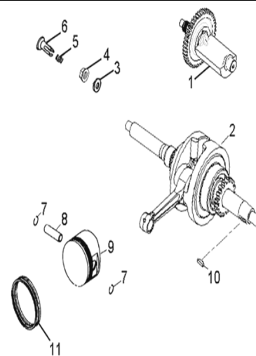
D-27: CRANKSHAFT & PISTON
