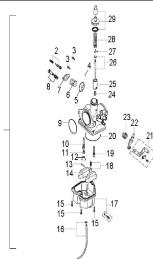
D-38: CARBURETOR
