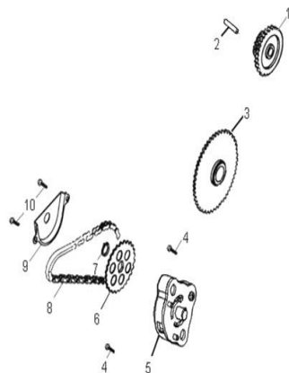
D-37: OIL PUMP
