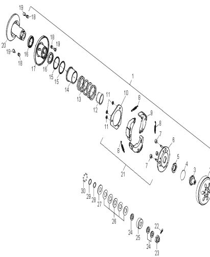
D-35: DRIVEN CLUTCH
