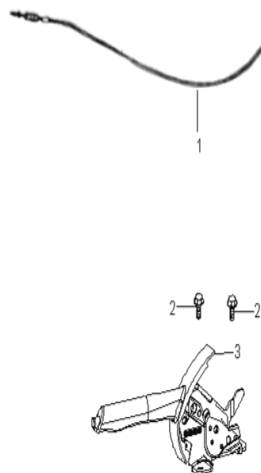
D-20: PARK BRAKE BLOCK
