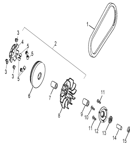
D-34: DRIVE CLUTCH
