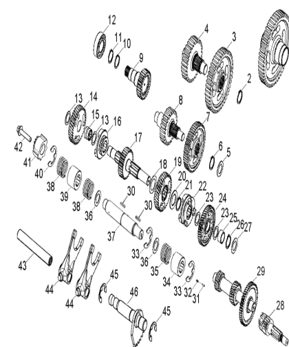
D-36: TRANSMISSION
