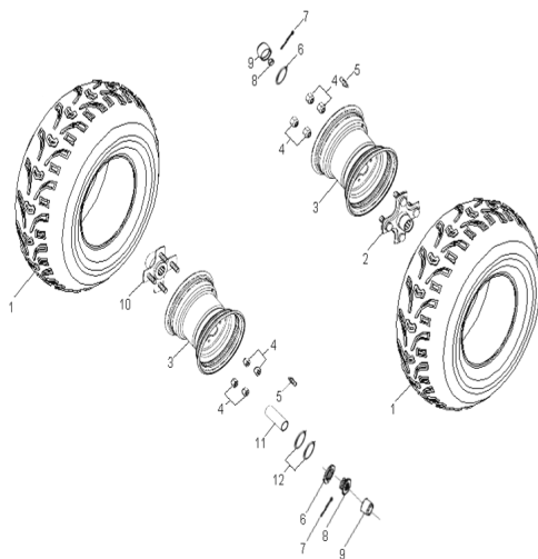
D-22: REAR WHEEL
