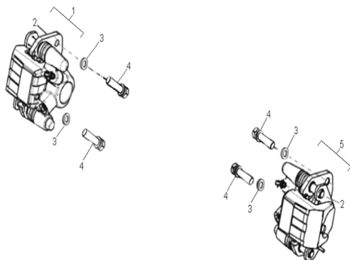
D-19: FRONT BRAKE CALIPER
