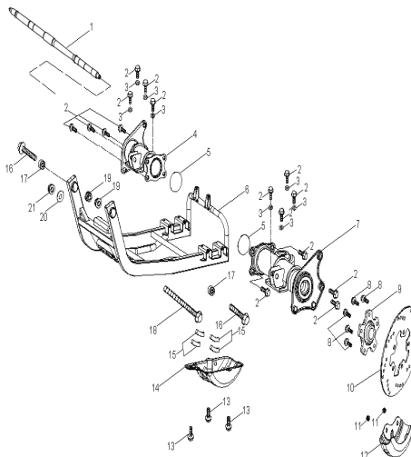
D-23: SWING ARM
