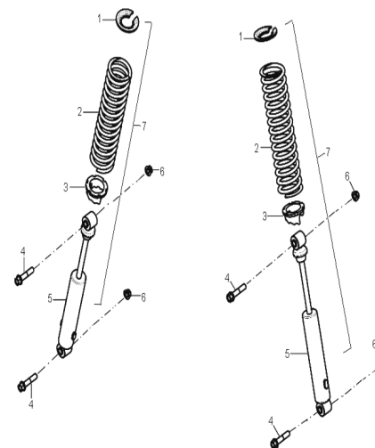
D-24: REAR SHOCK
