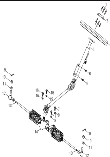
D-14: STEERING
