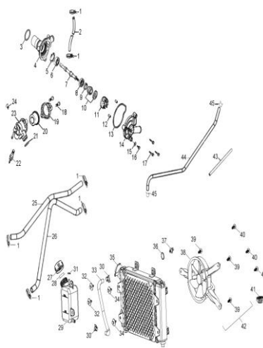
D-29: WATER PUMP & RADIATOR
