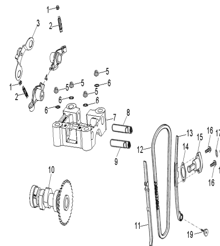
D-33: VALVE CAM
