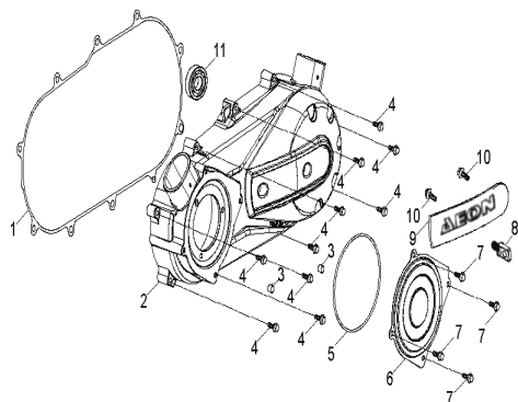
D-31: LEFT CRANKCASE COVER
