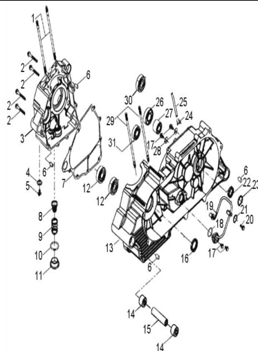
D-26: CRANKCASE
