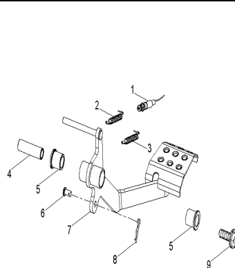
D-17: FOOT BRAKE
