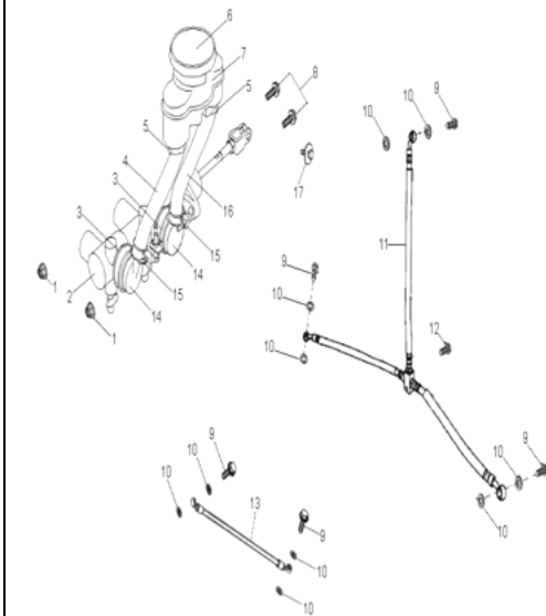
D-18: BRAKE LINES & MASTER CYLINDER
