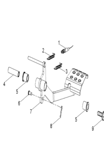
D-17: FOOT BRAKE
