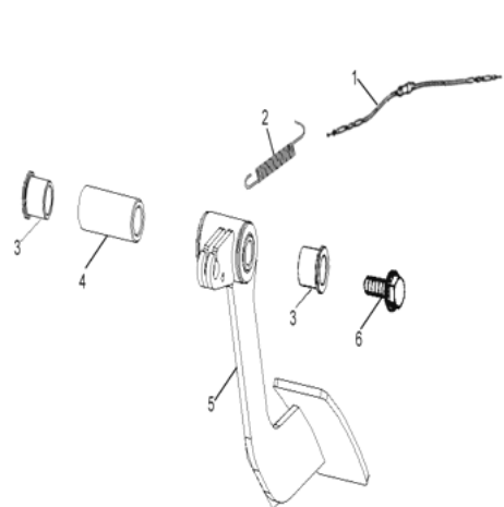
D-16: THROTTLE
