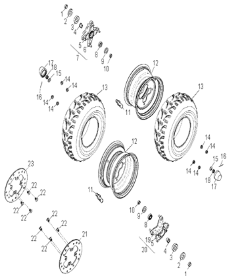
D-13: FRONT WHEEL
