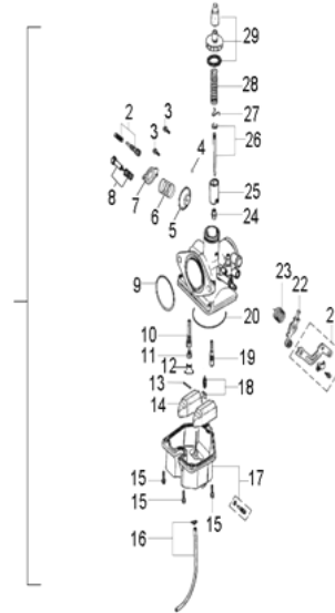
D-38: CARBURETOR
