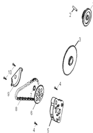
D-37: OIL PUMP
