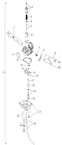
D-13: CARBURETOR
