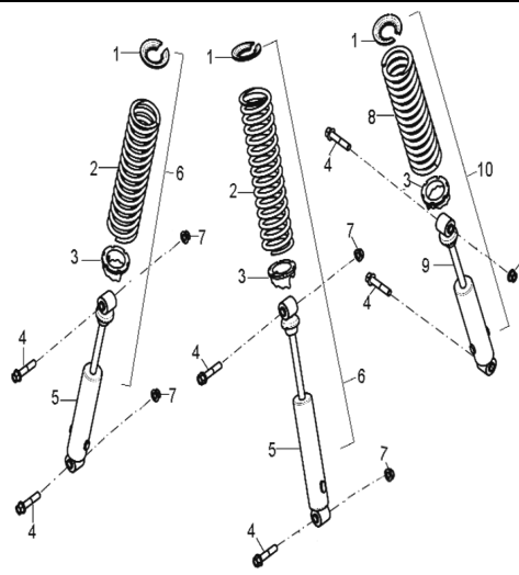
D-23: SUSPENSION
