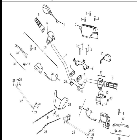
D-28: HANDLEBAR
