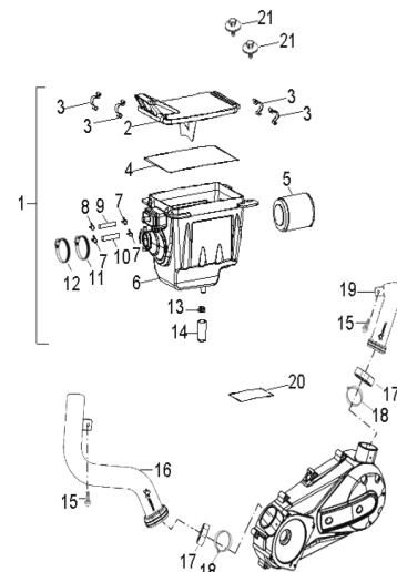
D-15: AIR CLEANER
