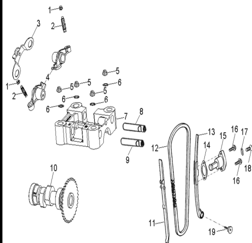
D-7: VALVE CAM
