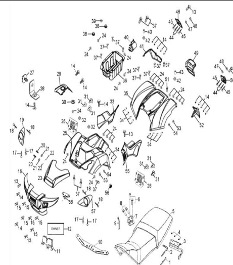
D-21: CAB &amp; SEAT
