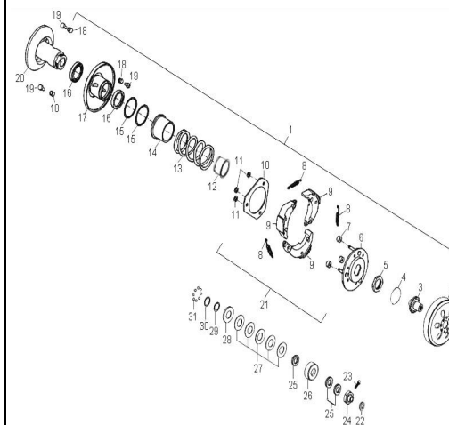
D-9: DRIVEN CLUTCH
