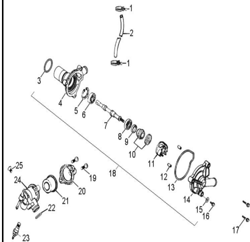
D-12: WATER PUMP
