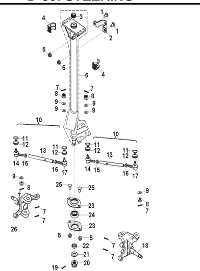
D-30: STEERING
