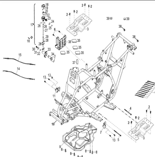
D-17: FRAME BODY
