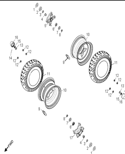
D-24: FRONT WHEEL
