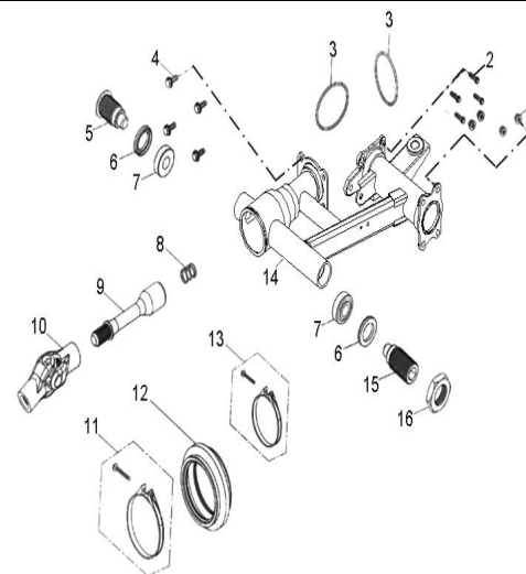
D-18: REAR SWIM ARM ASSEMBLY
