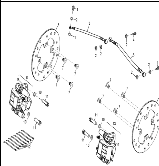
D-26: FRONT BRAKE
