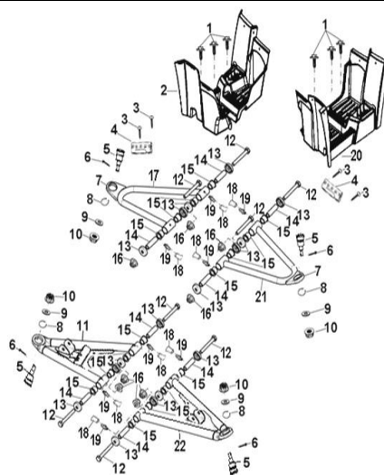
D-20: SWING ARM &amp; FOOTREST
