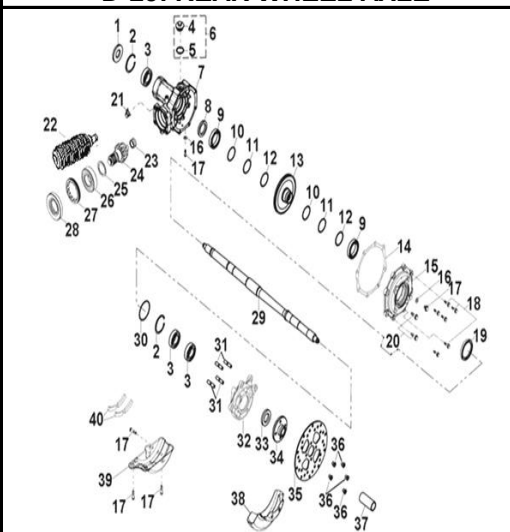
D-29: REAR WHEEL AXLE
