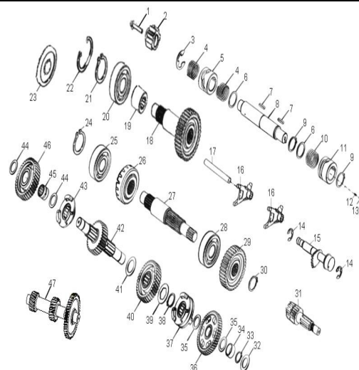
D-11: TRANSMISSION
