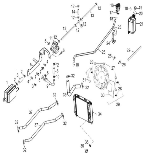
D-14: RADIATOR
