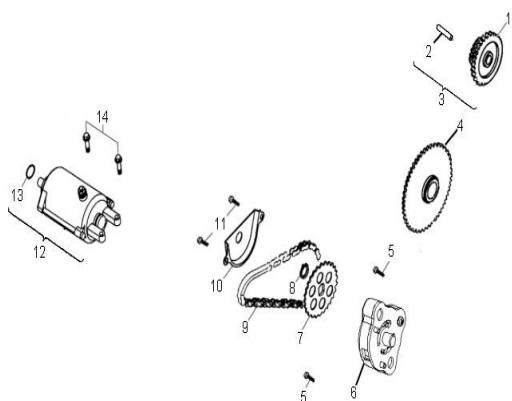
D-10: OIL PUMP &amp; STARTING MOTOR
