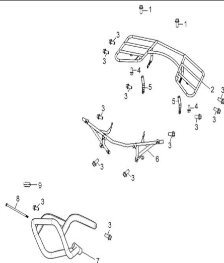
D-19: BUMPER
