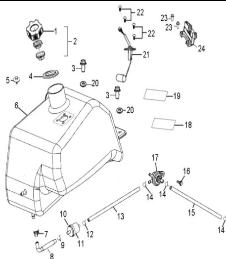
D-22: FUEL TANK
