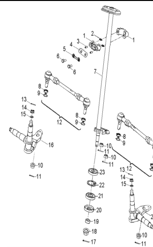
D-30: STEERING
