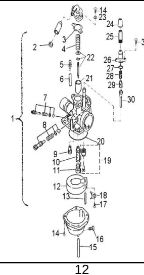
D-6: CARBURETOR
