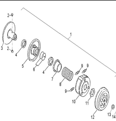
D-12: DRIVEN CLUTCH
