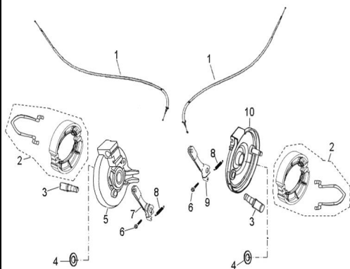
D-25: FRONT BRAKE
