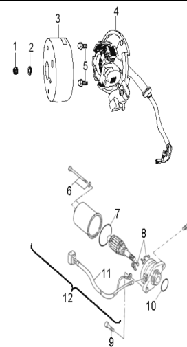
D-15: GENERATOR & START MOTOR
