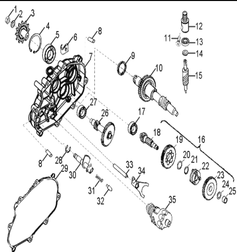
D-7: DRIVE SHAFT
