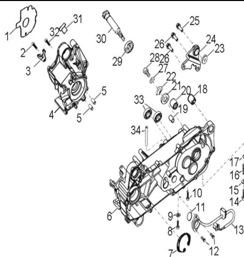
D-8: CRANKCASE
