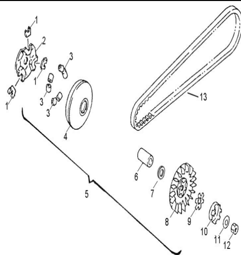
D-11: DRIVE CLUTCH
