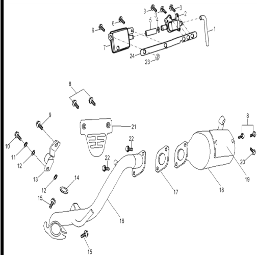
D-16: EXHAUST PIPE
