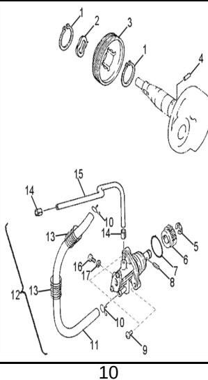
D-4: OIL PUMP
