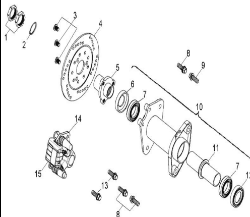
D-26: REAR BRAKE
