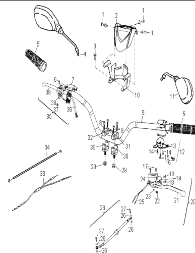
D-27: HANDLEBAR
