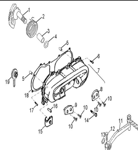
D-9: LEFT CRANKCASE COVER
