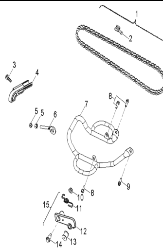
D-29: CHAIN
