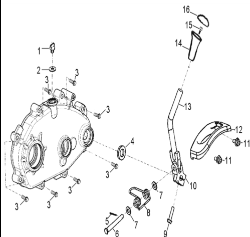
D-13: TRANSMISSION LEVER
