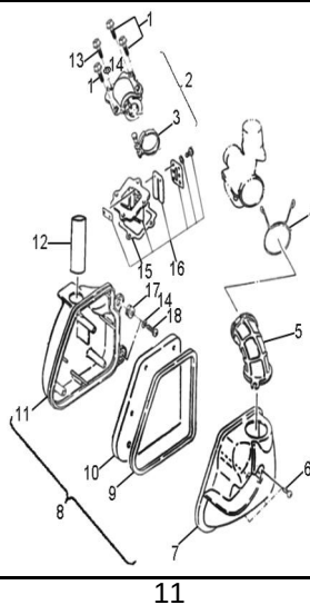
D-5: AIR CLEANER
