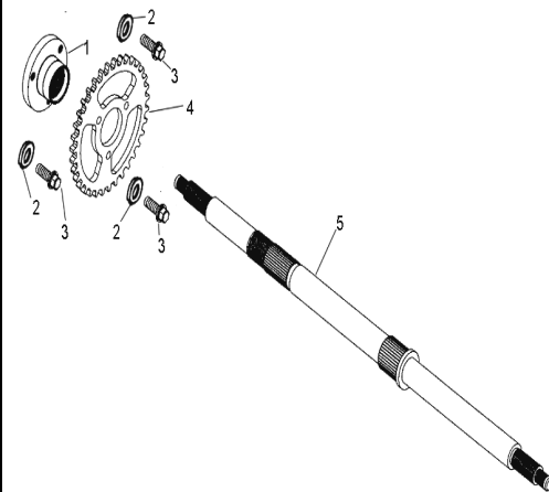
D-28: REAR WHEEL AXLE
