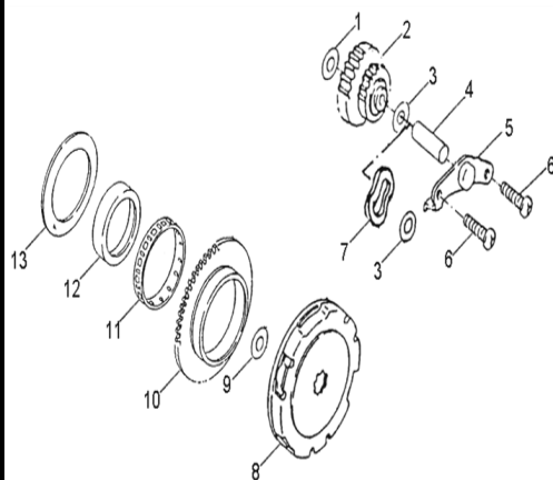
D-10: STARTER
