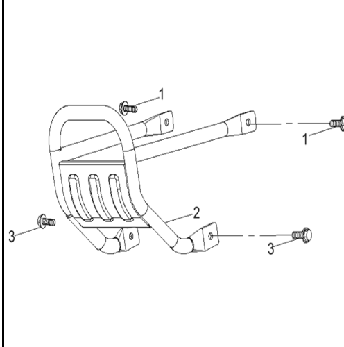
D-17: BUMPER
