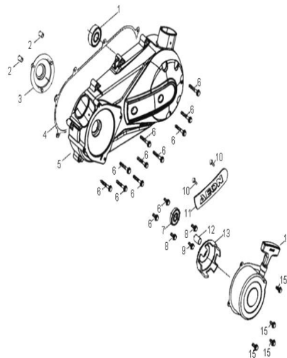
D-5: LEFT CRANKCASE COVER
