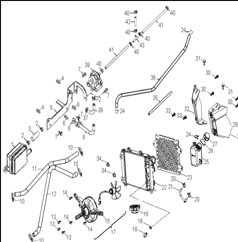
D-14: RADIATOR
