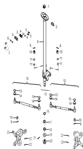
D-30: STEERING
