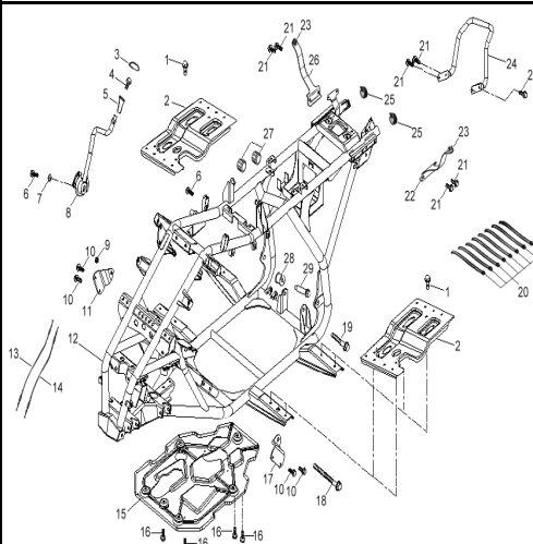
D-17: FRAME BODY
