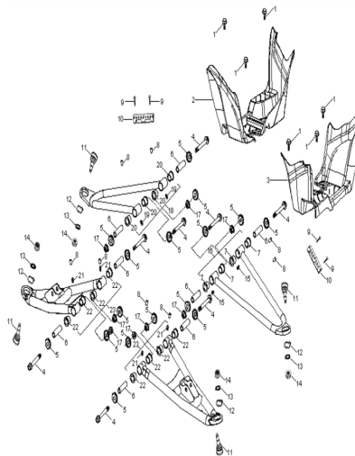
D-20: SWING ARM & FOOTREST
