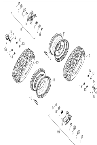
D-24: FRONT WHEEL
