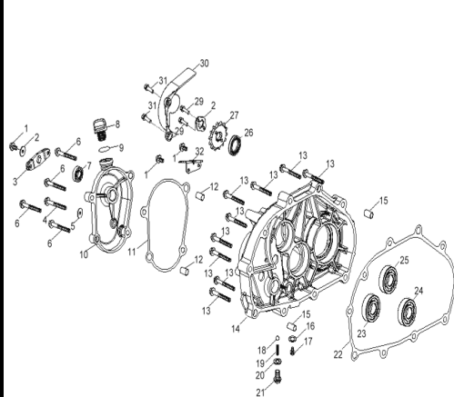
D-4: REAR DRIVE ASSEMBLY
