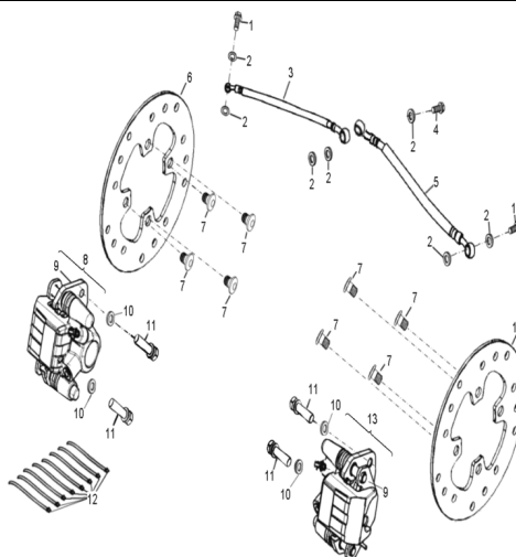
D-26: FRONT BRAKE
