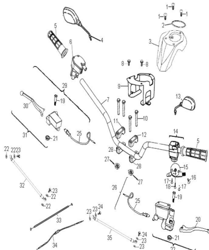
D-28: HANDLEBAR
