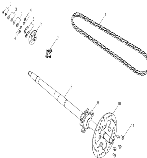
D-29: REAR WHEEL AXLE
