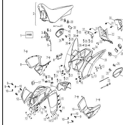
D-21: CAB & SEAT
