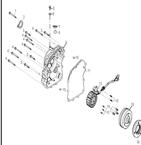
D-6: RIGHT CRANKCASE COVER
