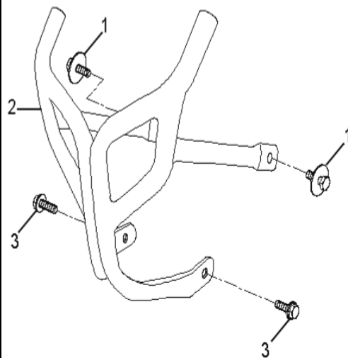
D-19: BUMPER
