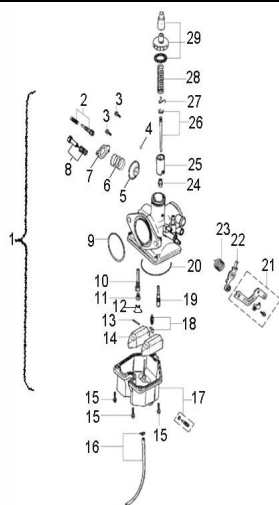
D-13: CARBURETOR
