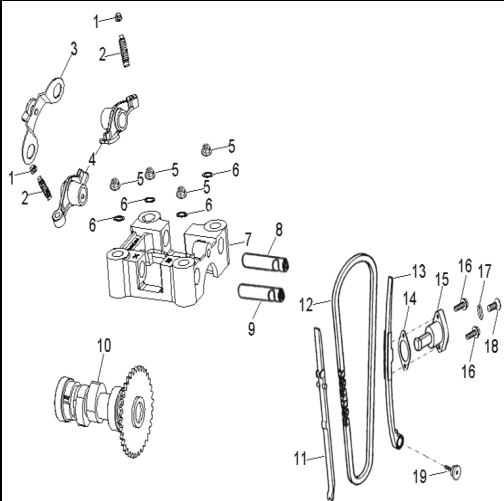
D-7: VALVE CAM
