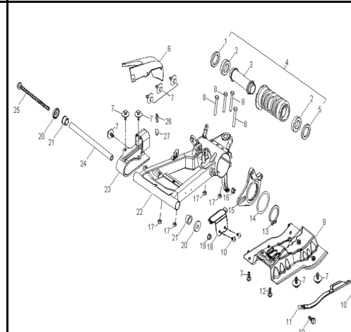
D-18: REAR SWIM ARM ASSEMBLY
