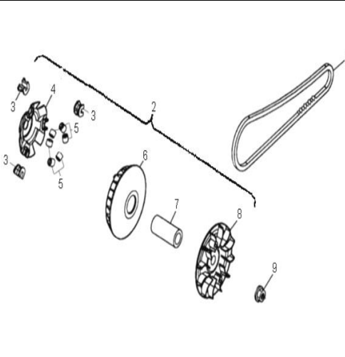
D-8: DRIVE CLUTCH
