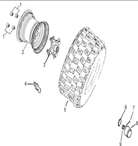
D-25: REAR WHEEL
