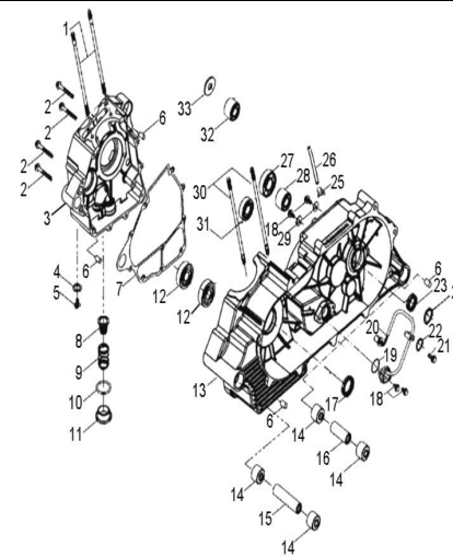
D-3: CRANKCASE
