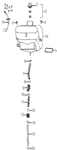
D-22: FUEL TANK
