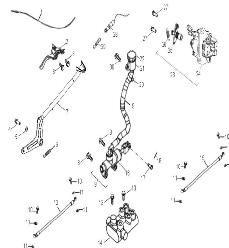
D-27: REAR BRAKE
