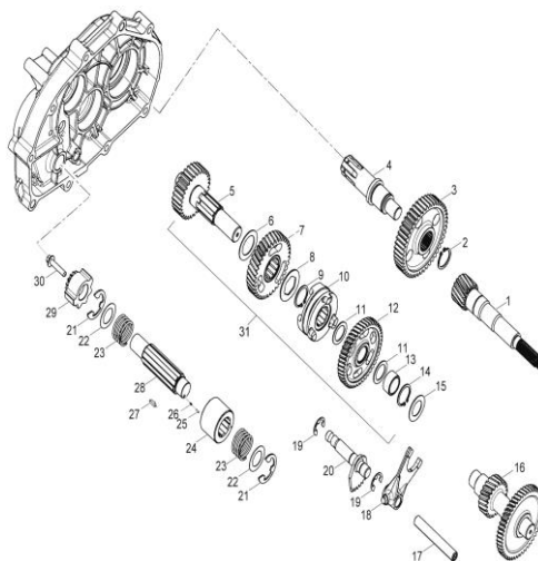
D-11: TRANSMISSION
