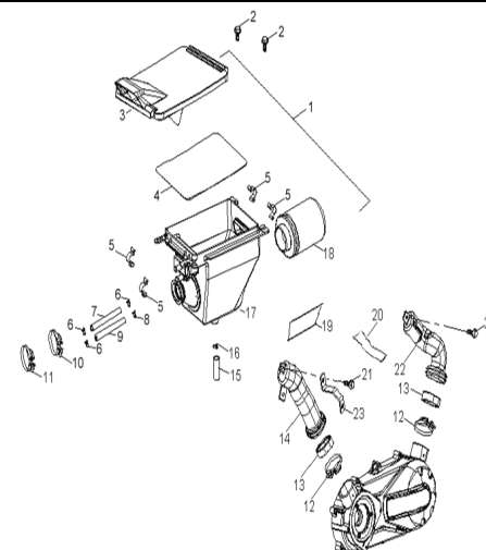
D-15: AIR CLEANER
