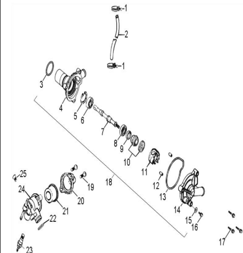
D-12: WATER PUMP
