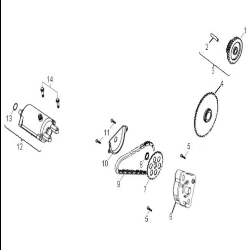
D-10: OIL PUMP & STARTING MOTOR
