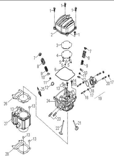
D-1: CYLINDER HEAD
