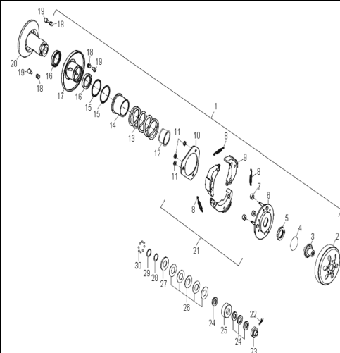
D-9: DRIVEN CLUTCH
