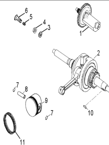
D-2: PISTON , CRANKSHAFT
