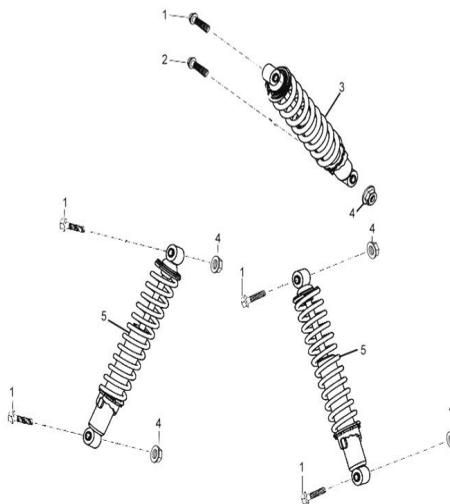
D-23: SUSPENSION
