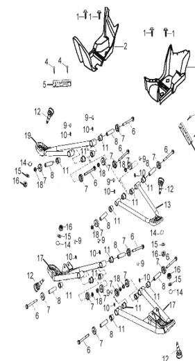
D-18: SWING ARM & FOOTREST
