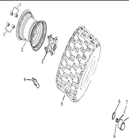
D-23: REAR WHEEL
