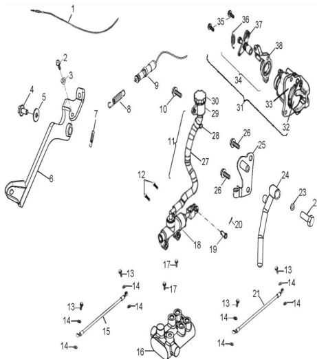
D-25: REAR BRAKE
