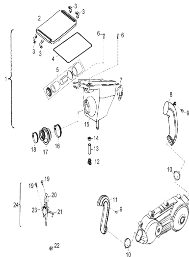
D-13: AIR CLEANER
