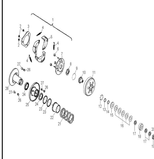
D-9: DRIVEN CLUTCH
