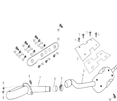
D-14: EXHAUST PIPE
