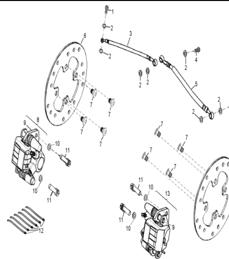
D-24: FRONT BRAKE
