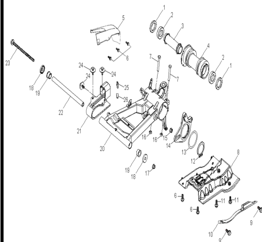
D-16: REAR SWIM ARM ASSEMBLY
