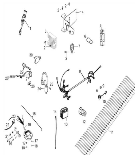
D-30: ELECTRICAL PARTS
