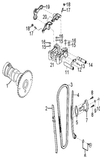
D-7: VALVE CAM
