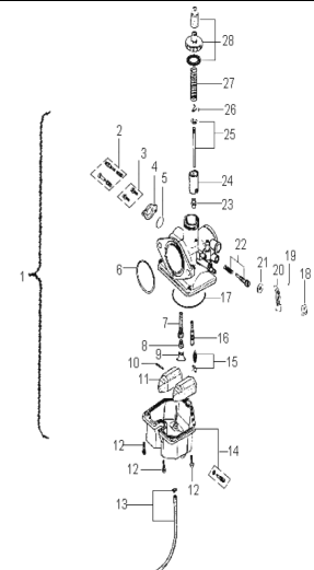
D-12: CARBURETOR
