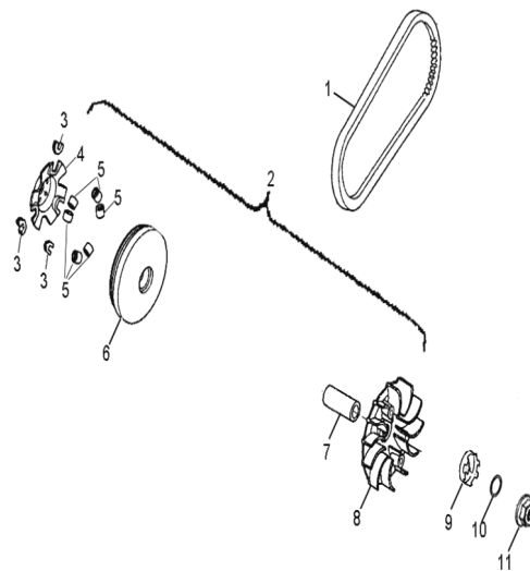
D-8: DRIVE CLUTCH
