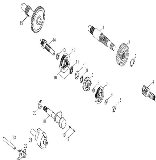
D-11: TRANSMISSION
