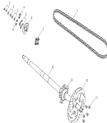
D-27: REAR WHEEL AXLE
