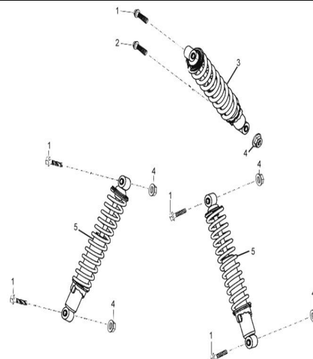
D-21: SUSPENSION
