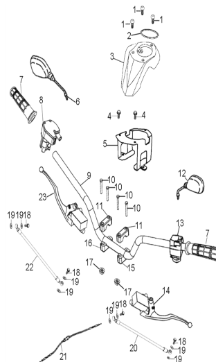
D-26: HANDLEBAR
