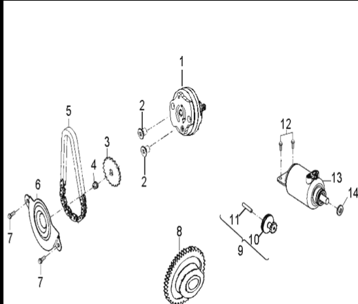
D-10: OIL PUMP & STARTING MOTOR
