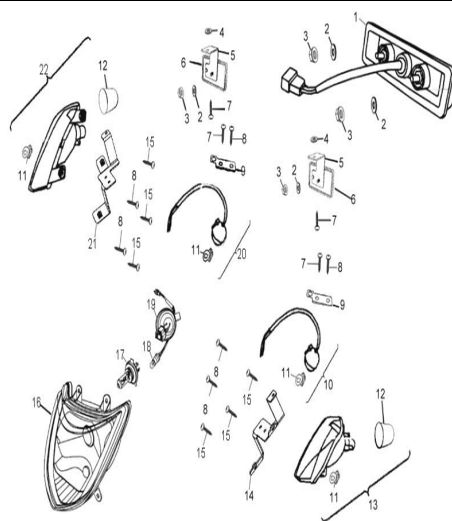
D-29: LIGHTS
