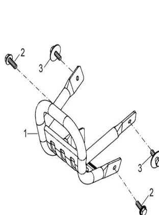
D-17: BUMPER
